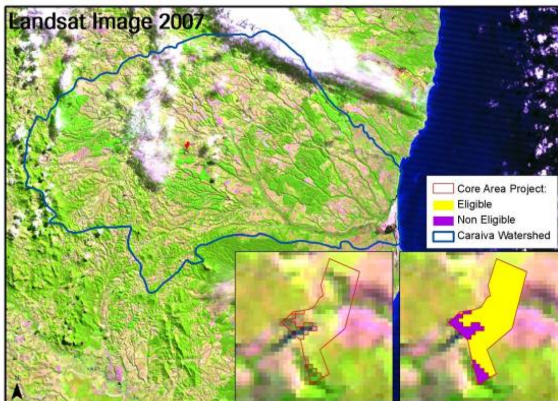
Figure 13: Land use classification – 2007. Forest areas in green
